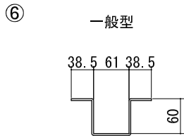
母屋取付板A t=2.3
